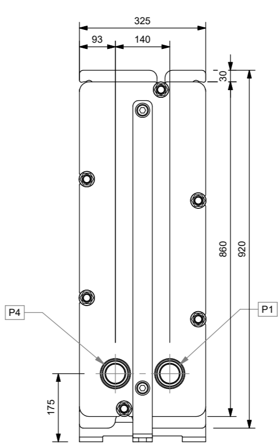
BACK VIEW SCALE 1 : 10
