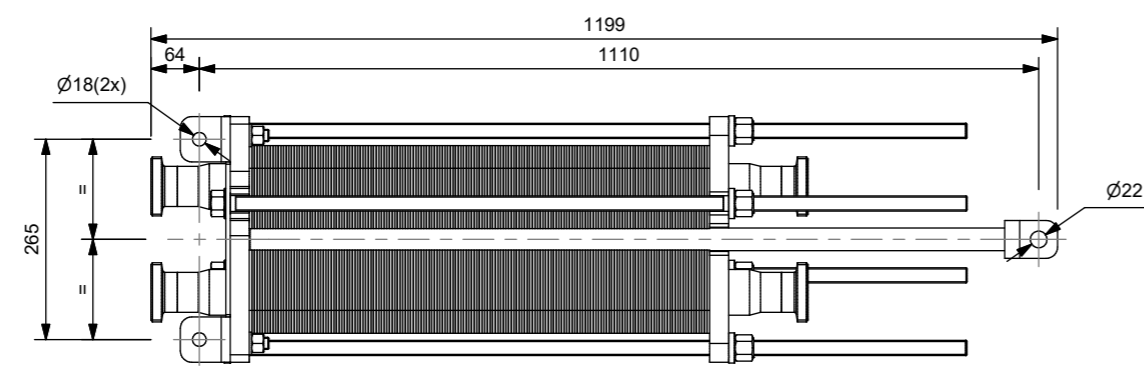
BOTTOM VIEW SCALE 1 : 10
