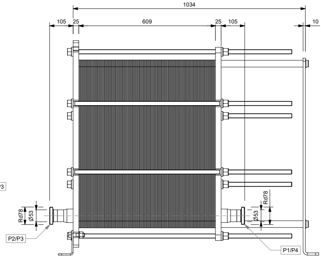
RIGHT VIEW SCALE 1 : 10
