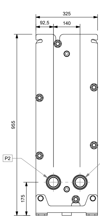
FRONT VIEW SCALE 1 : 10
